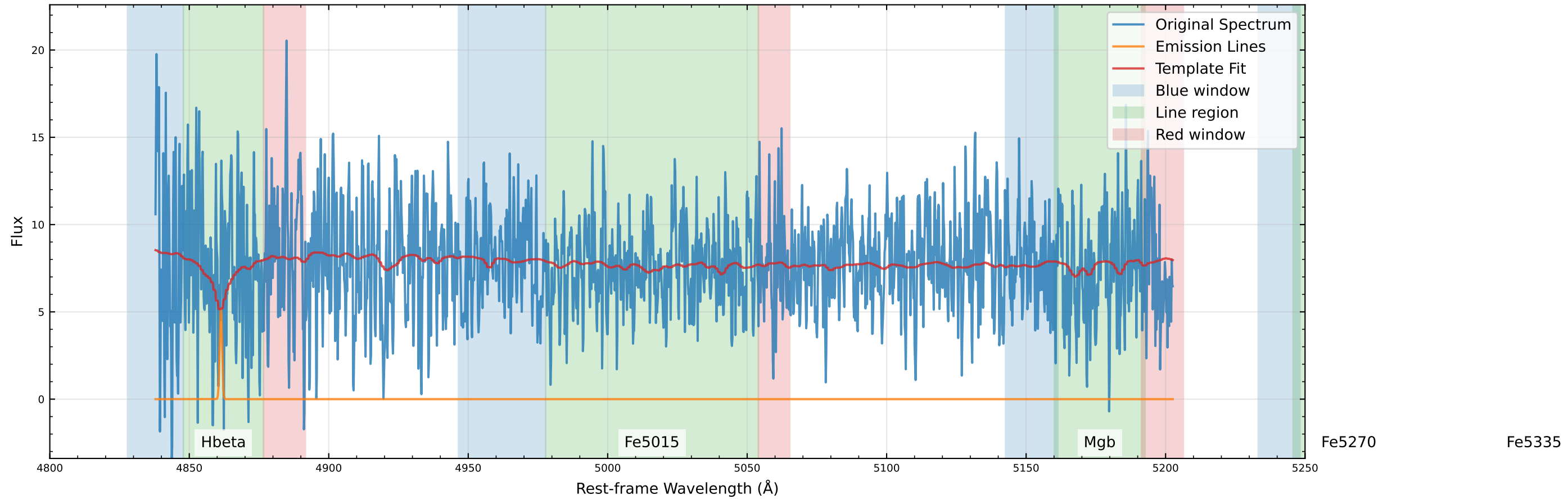
Original Data Comparison (v_star=-18.0 km/s, v_gas=12.9 km/s)
