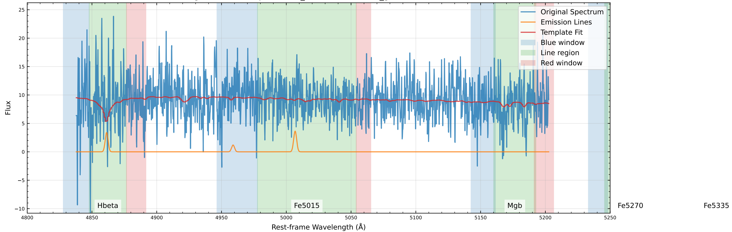
Original Data Comparison (v_star=68.8 km/s, v_gas=116.5 km/s)
