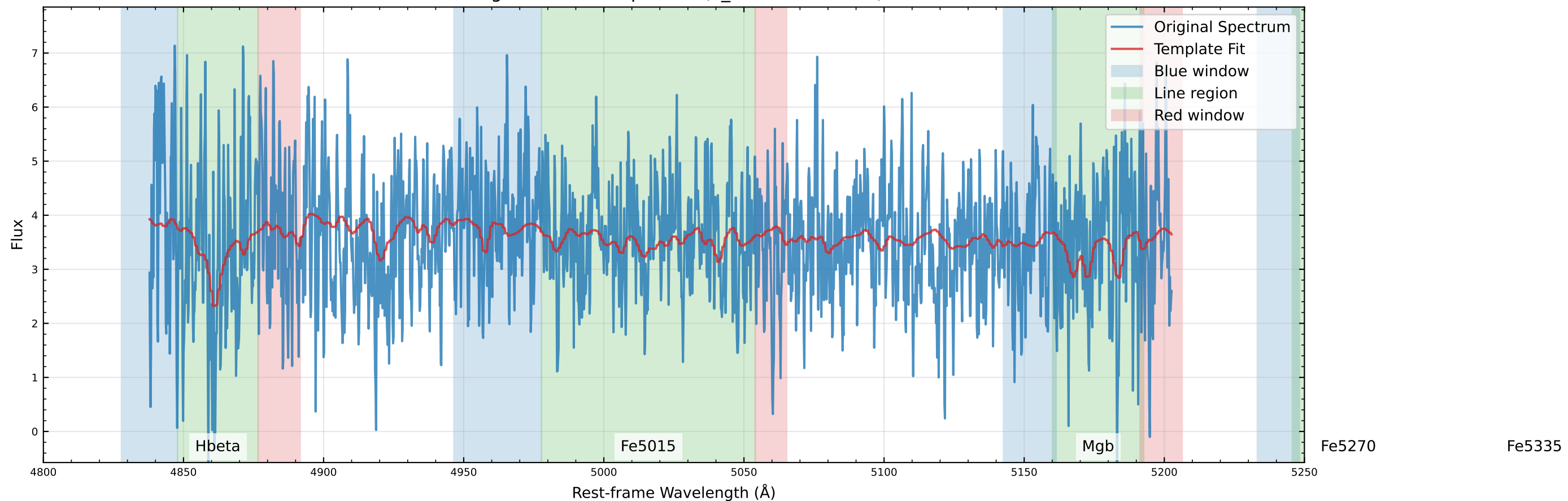
Original Data Comparison (v_star=-43.6 km/s)
