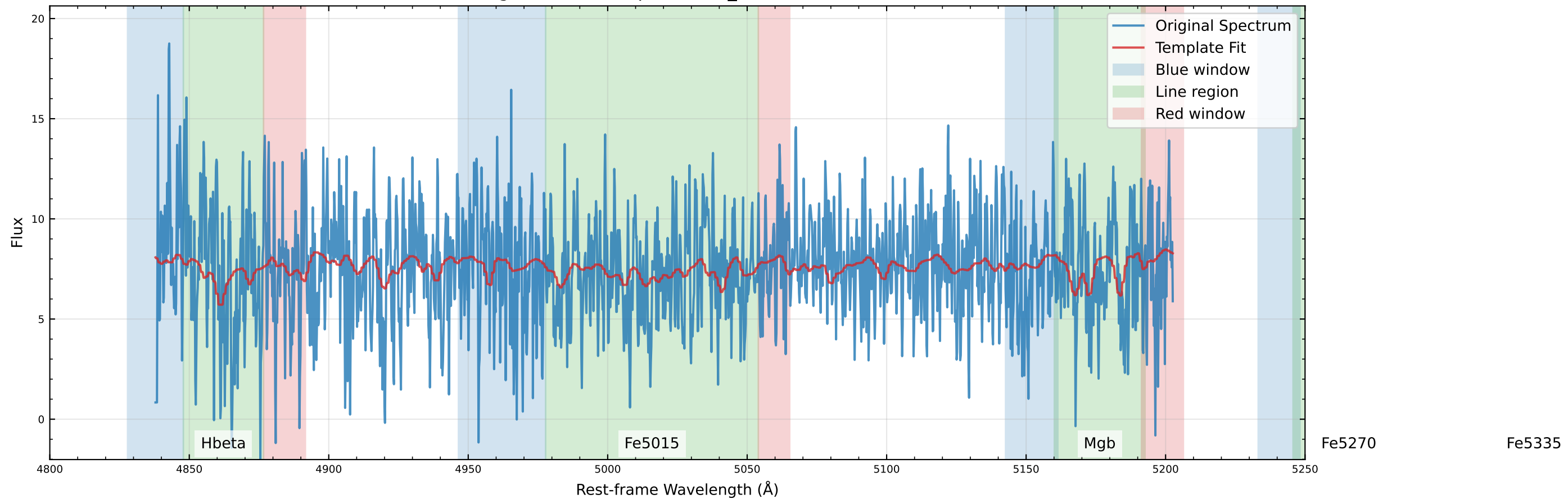
Original Data Comparison (v_star=73.0 km/s)
