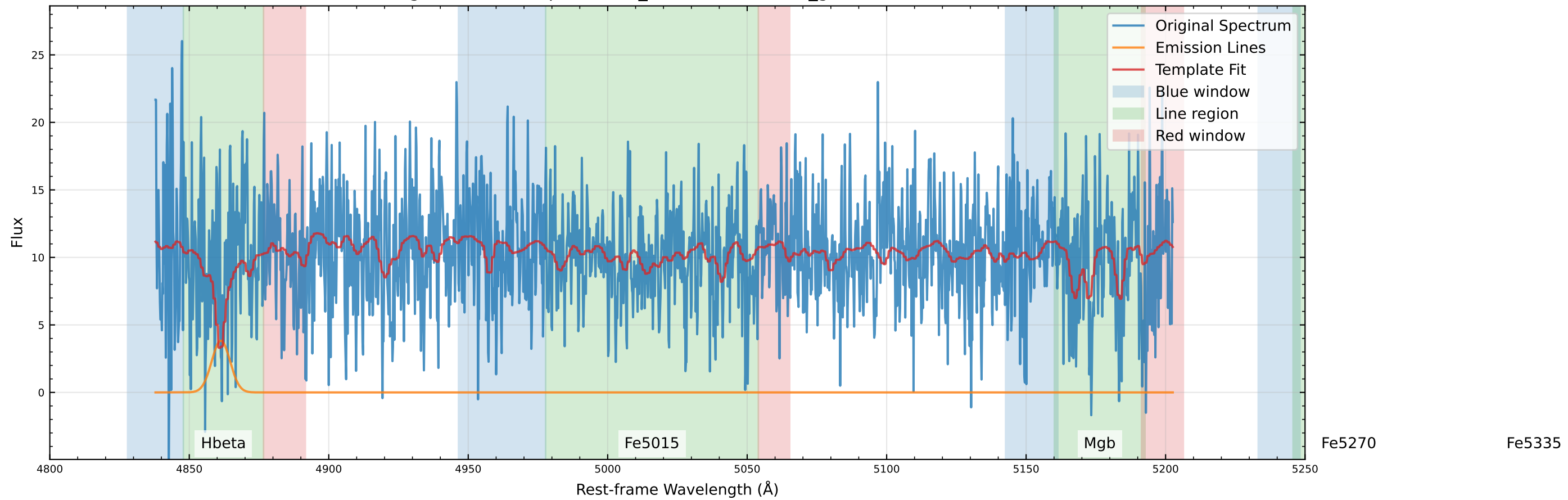
Original Data Comparison (v_star=18.5 km/s, v_gas=151.9 km/s)
