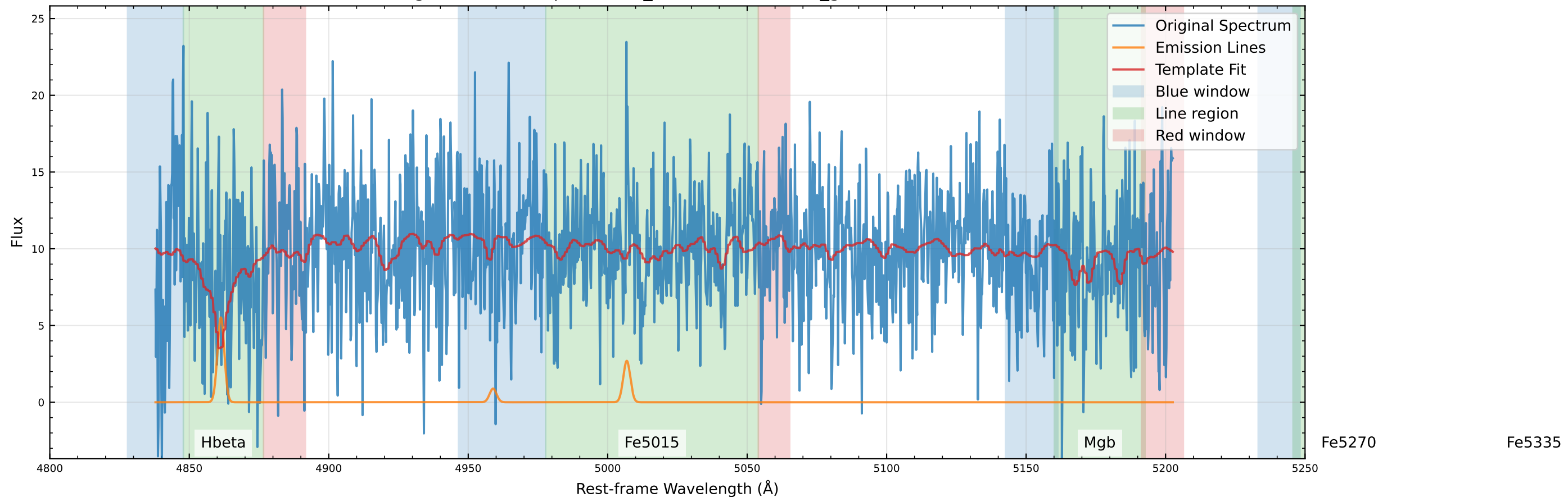
Original Data Comparison (v_star=-22.3 km/s, v_gas=-2.8 km/s)
