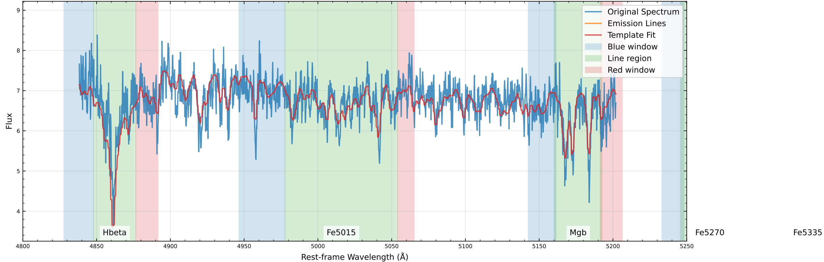
Original Data Comparison (v_star=18.2 km/s, v_gas=16.3 km/s)
