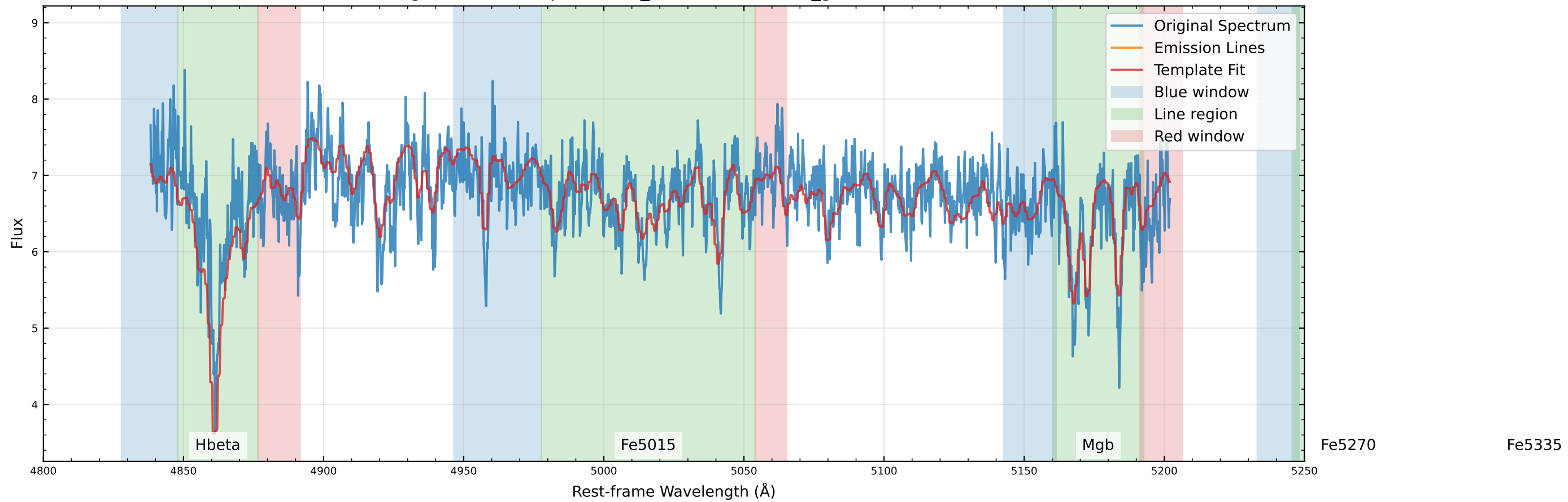
Original Data Comparison (v_star=18.2 km/s, v_gas=16.3 km/s)
