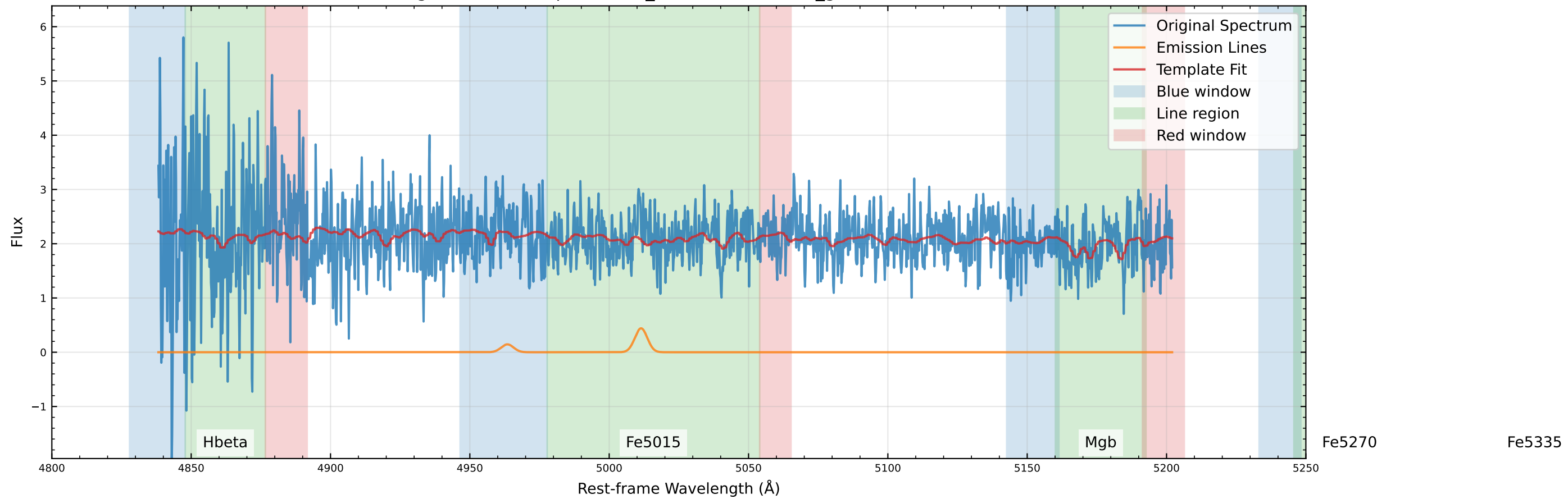
Original Data Comparison (v_star=14.5 km/s, v_gas=14.5 km/s)
