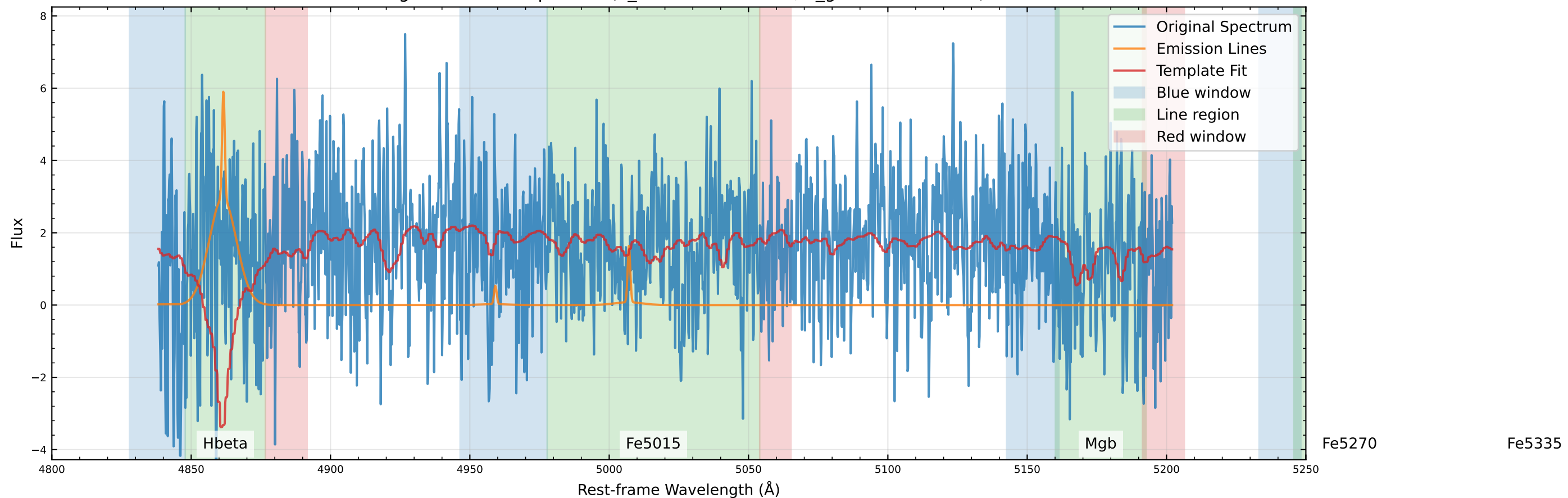
Original Data Comparison (v_star=-354.8 km/s, v_gas=-470.8 km/s)
