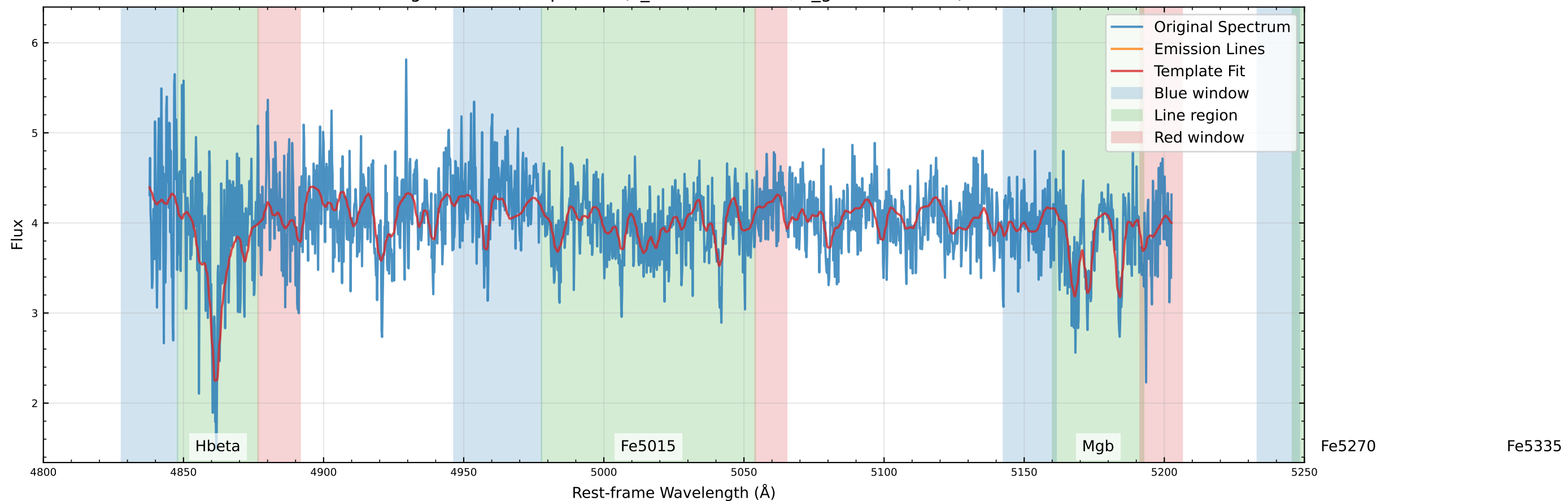
Original Data Comparison (v_star=19.9 km/s, v_gas=65.6 km/s)
