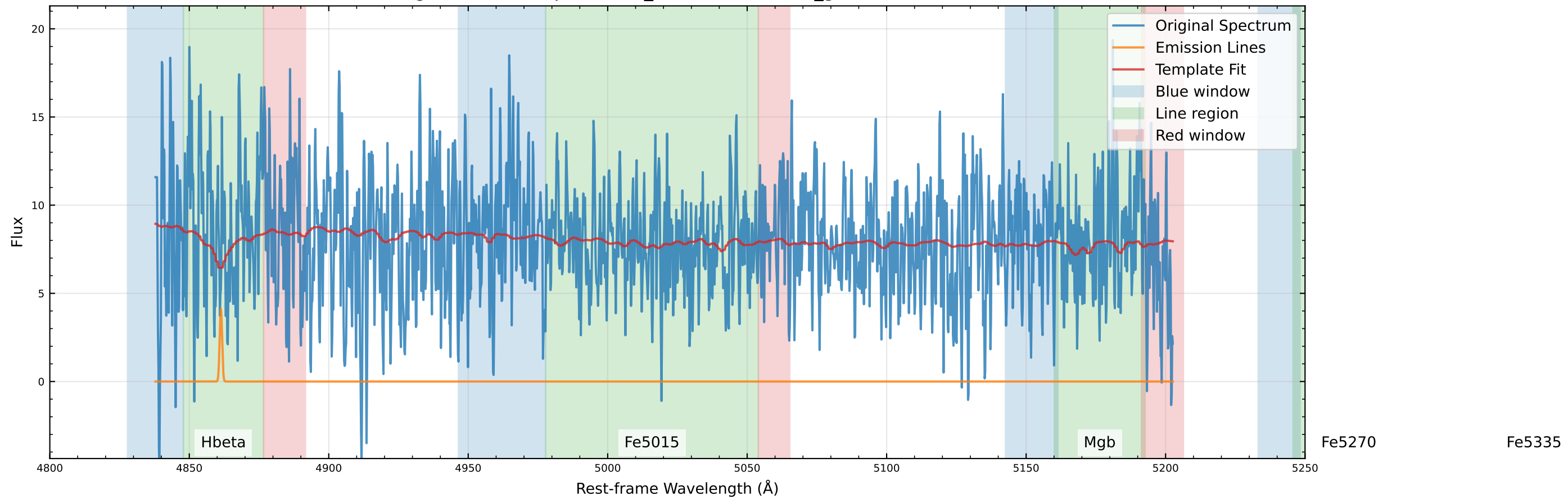
Original Data Comparison (v_star=63.9 km/s, v_gas=44.0 km/s)
