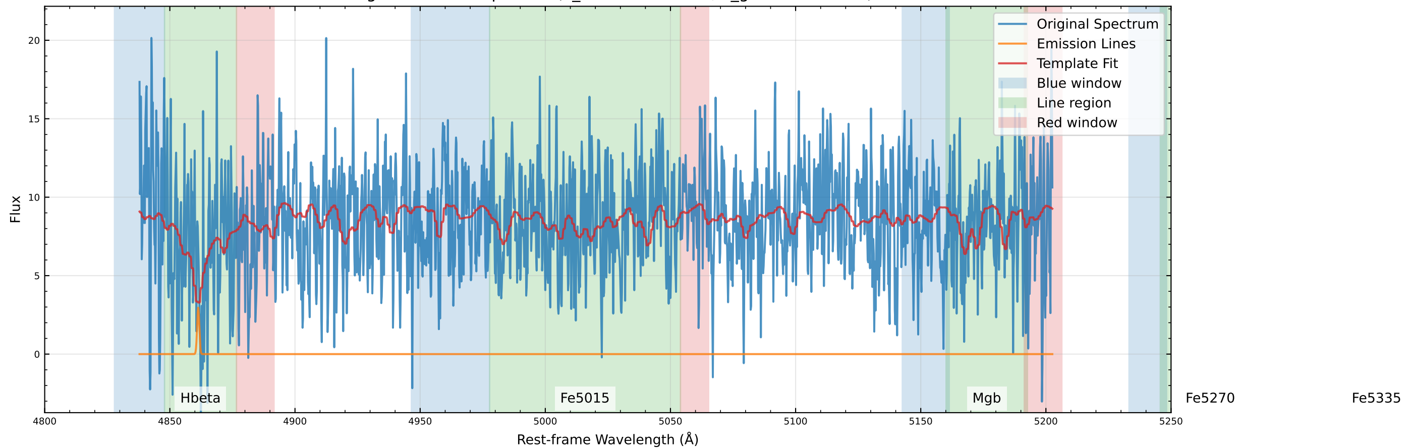
Original Data Comparison (v_star=-45.9 km/s, v_gas=-83.7 km/s)
