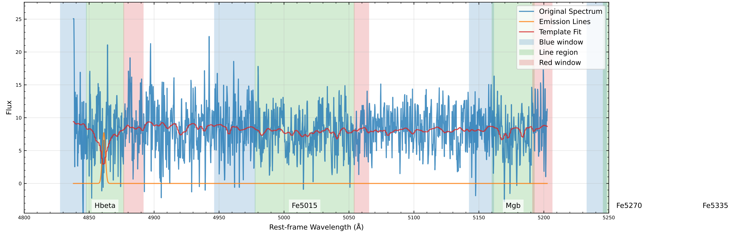
Original Data Comparison (v_star=57.3 km/s, v_gas=159.9 km/s)
