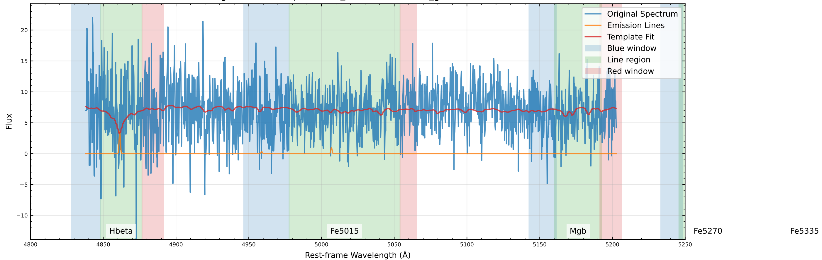
Original Data Comparison (v_star=58.5 km/s, v_gas=47.1 km/s)
