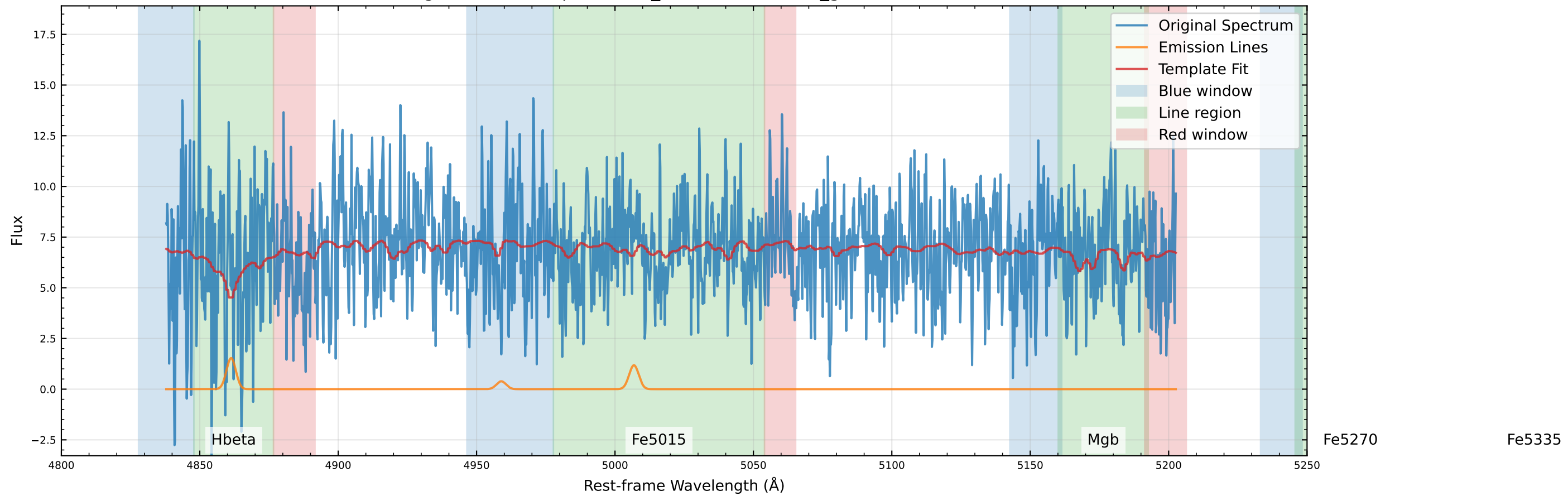
Original Data Comparison (v_star=37.8 km/s, v_gas=12.0 km/s)
