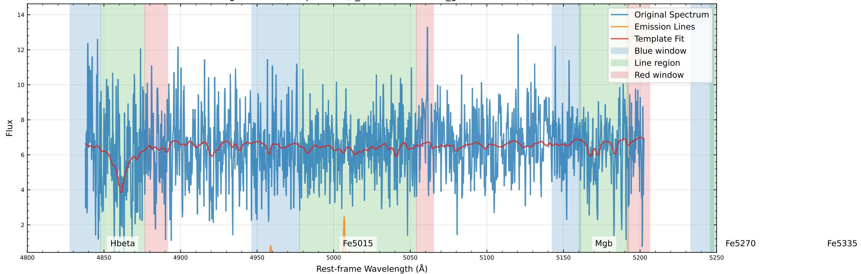
Original Data Comparison (v_star=-6.8 km/s, v_gas=70.3 km/s)
