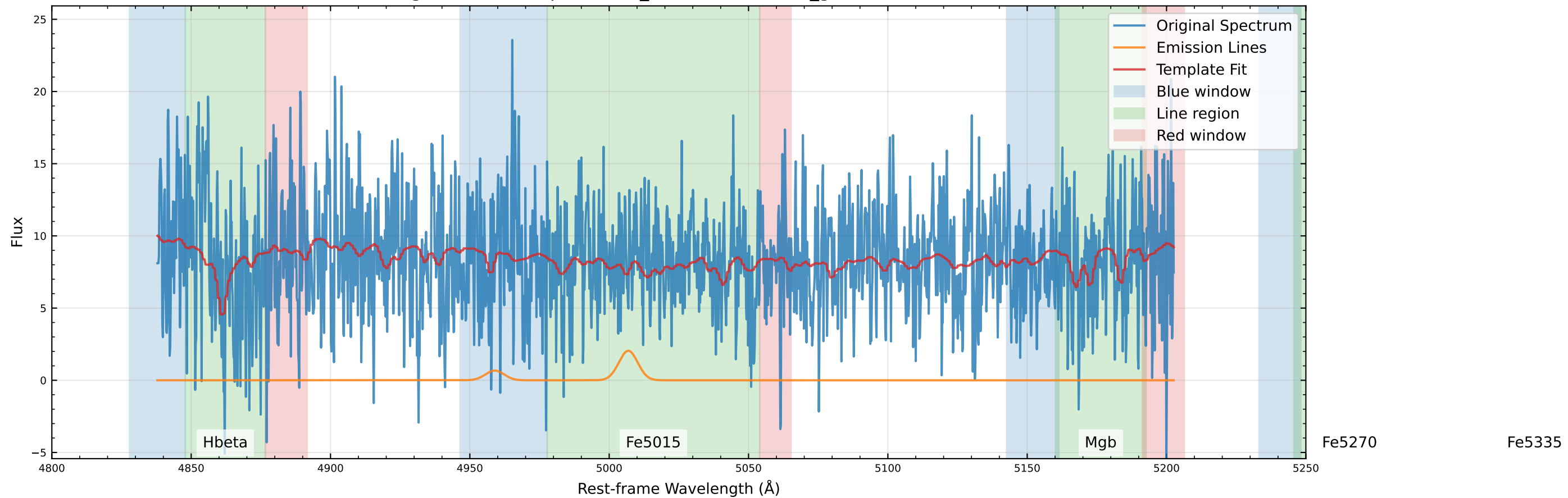
Original Data Comparison (v_star=63.5 km/s, v_gas=298.8 km/s)
