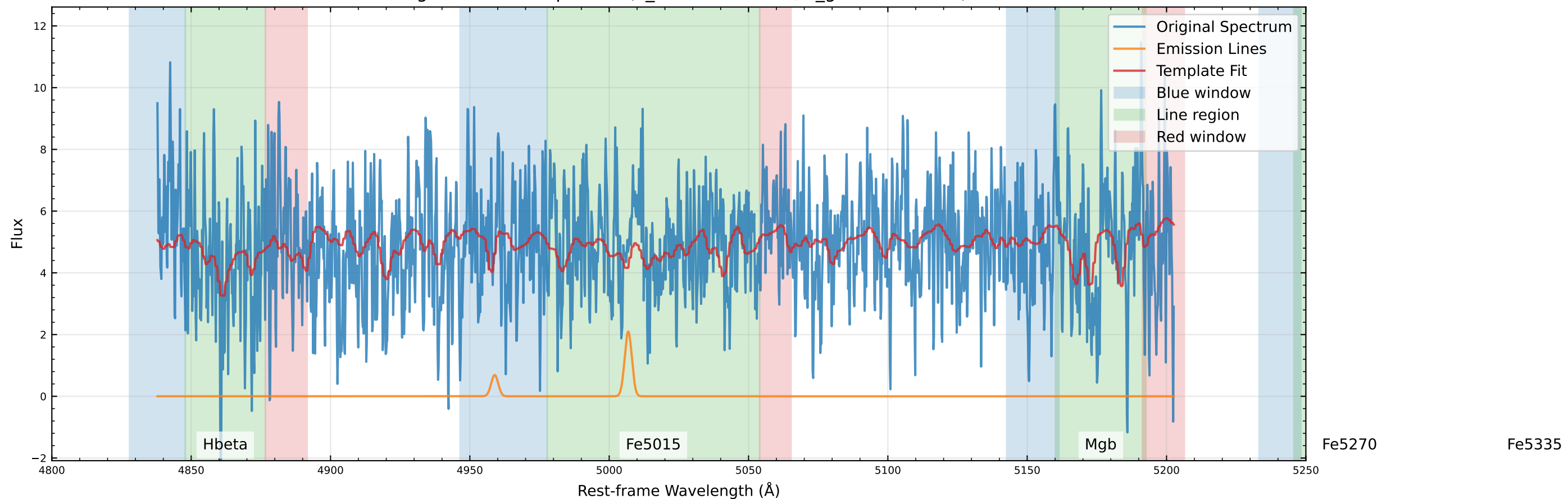
Original Data Comparison (v_star=80.0 km/s, v_gas=92.8 km/s)
