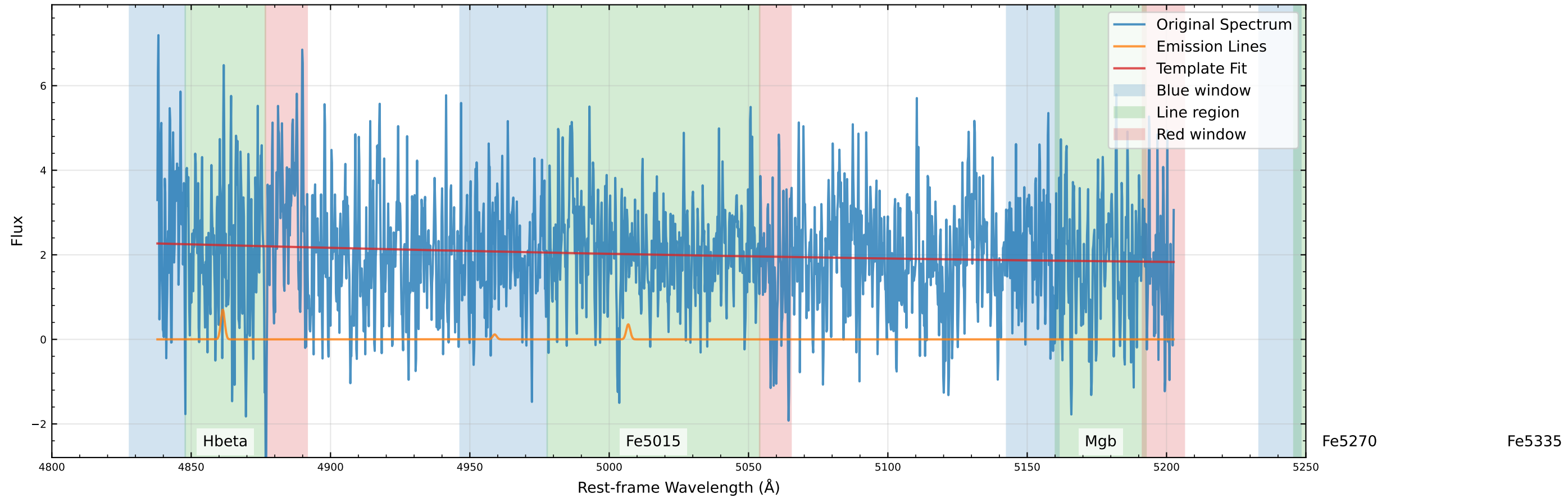
Original Data Comparison (v_star=0.0 km/s, v_gas=0.2 km/s)
