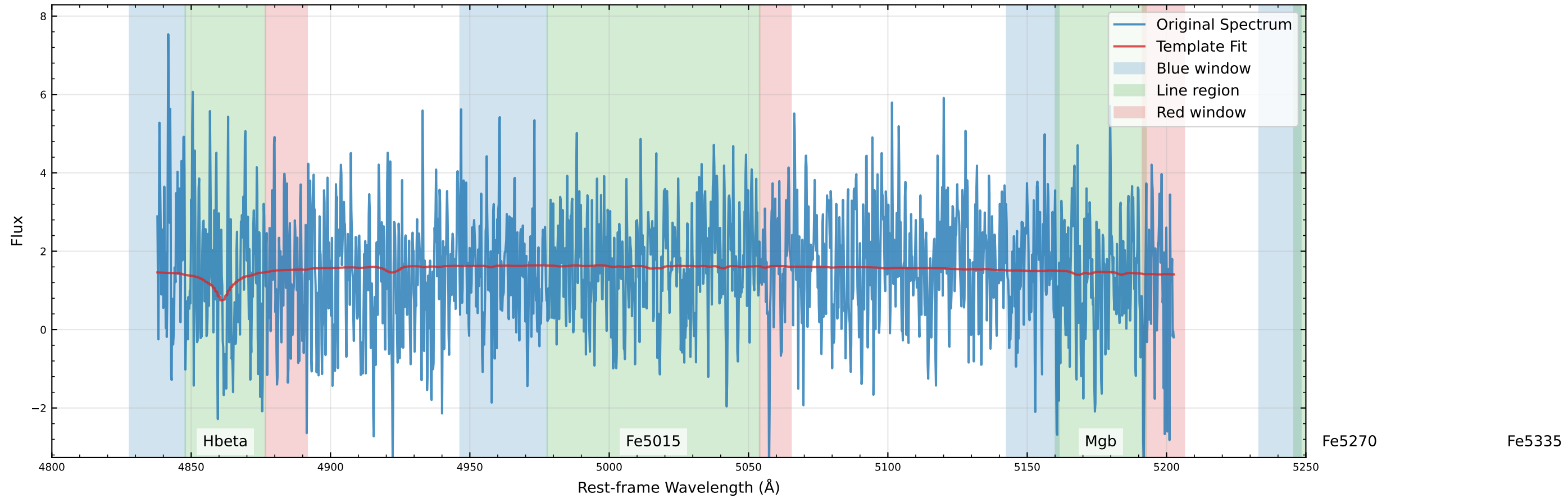
Original Data Comparison (v_star=66.3 km/s)
