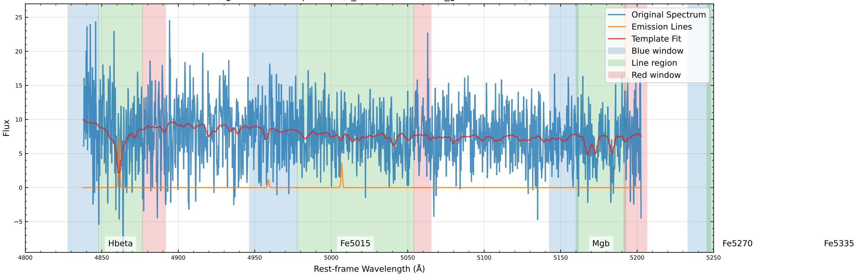
Original Data Comparison (v_star=46.2 km/s, v_gas=70.0 km/s)
