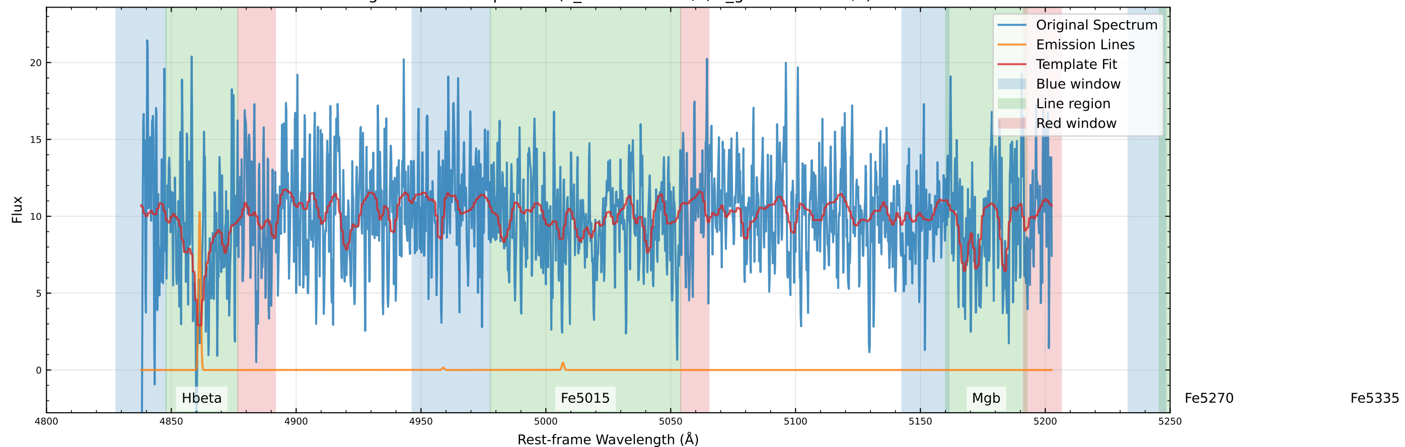
Original Data Comparison (v_star=47.9 km/s, v_gas=106.8 km/s)
