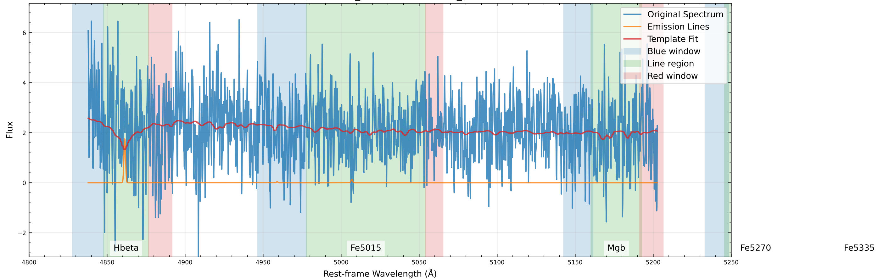
Original Data Comparison (v_star=521.0 km/s, v_gas=624.6 km/s)
