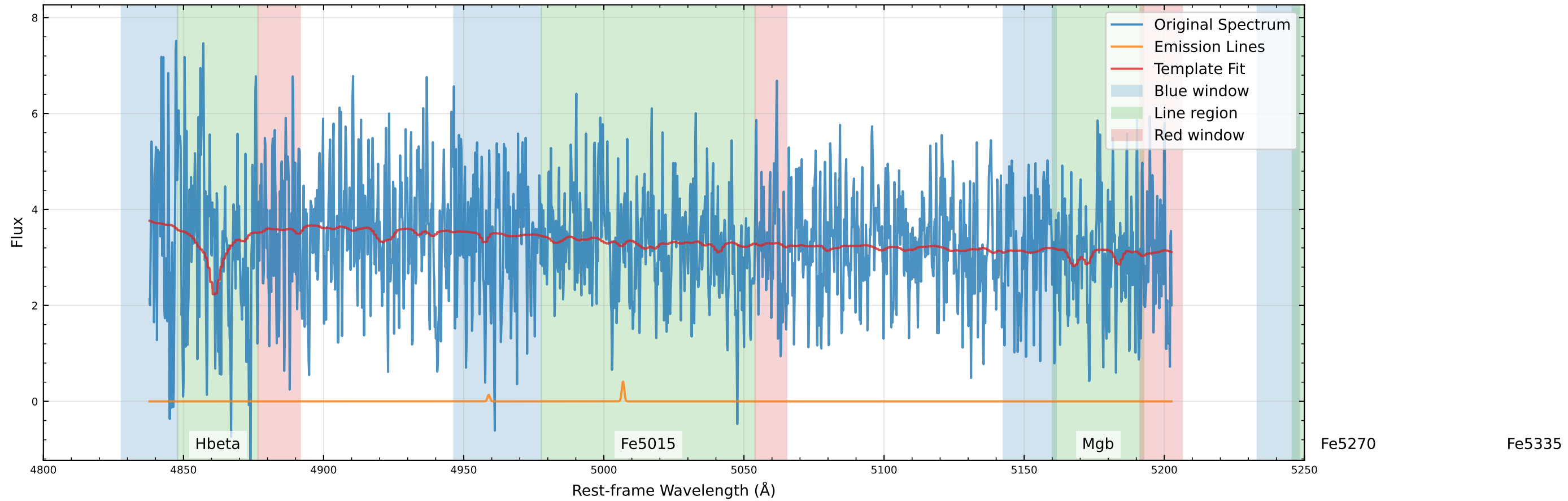
Original Data Comparison (v_star=65.3 km/s, v_gas=80.4 km/s)
