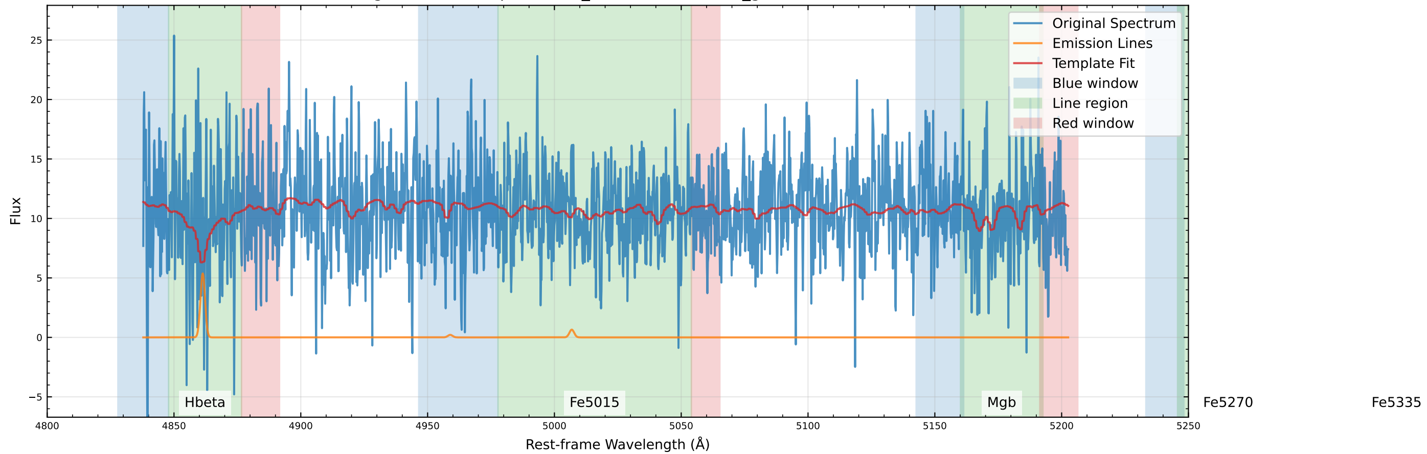
Original Data Comparison (v_star=-23.9 km/s, v_gas=-96.1 km/s)
