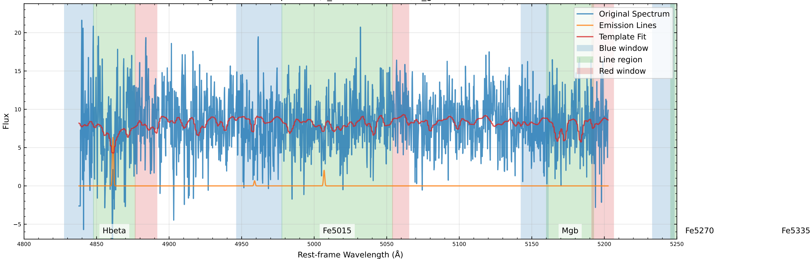
Original Data Comparison (v_star=128.9 km/s, v_gas=164.8 km/s)
