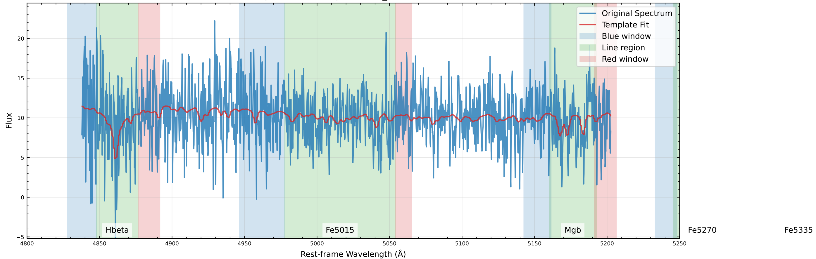
Original Data Comparison ( v_{\text{star}}=7.3 km/s)
