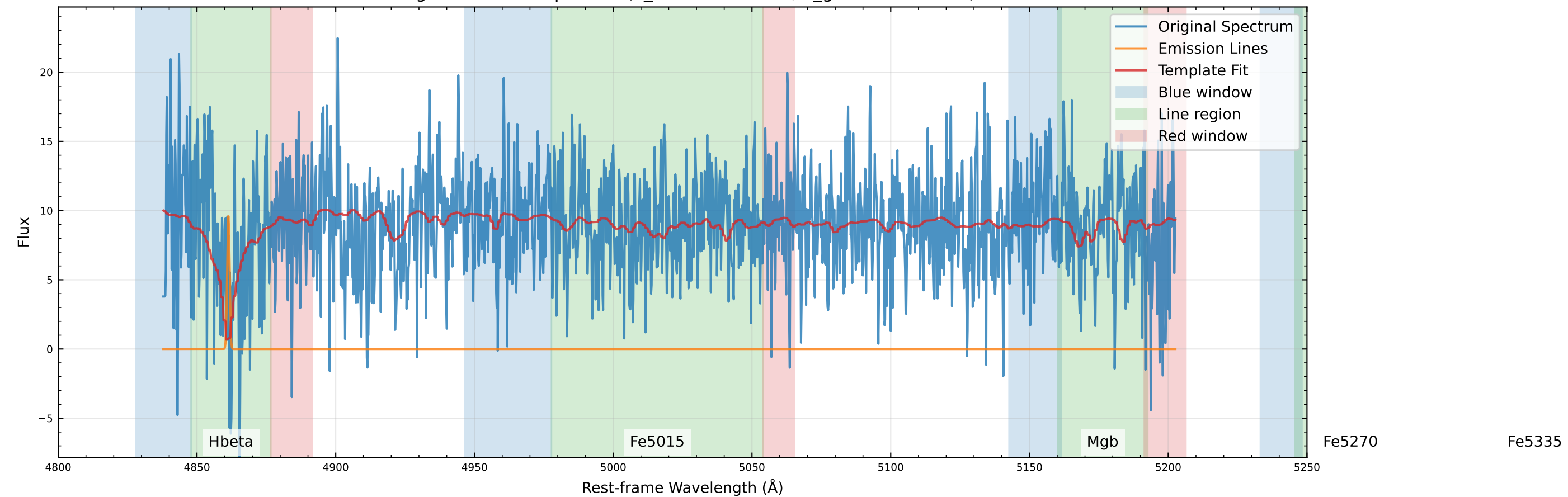
Original Data Comparison (v_star=84.6 km/s, v_gas=141.4 km/s)
