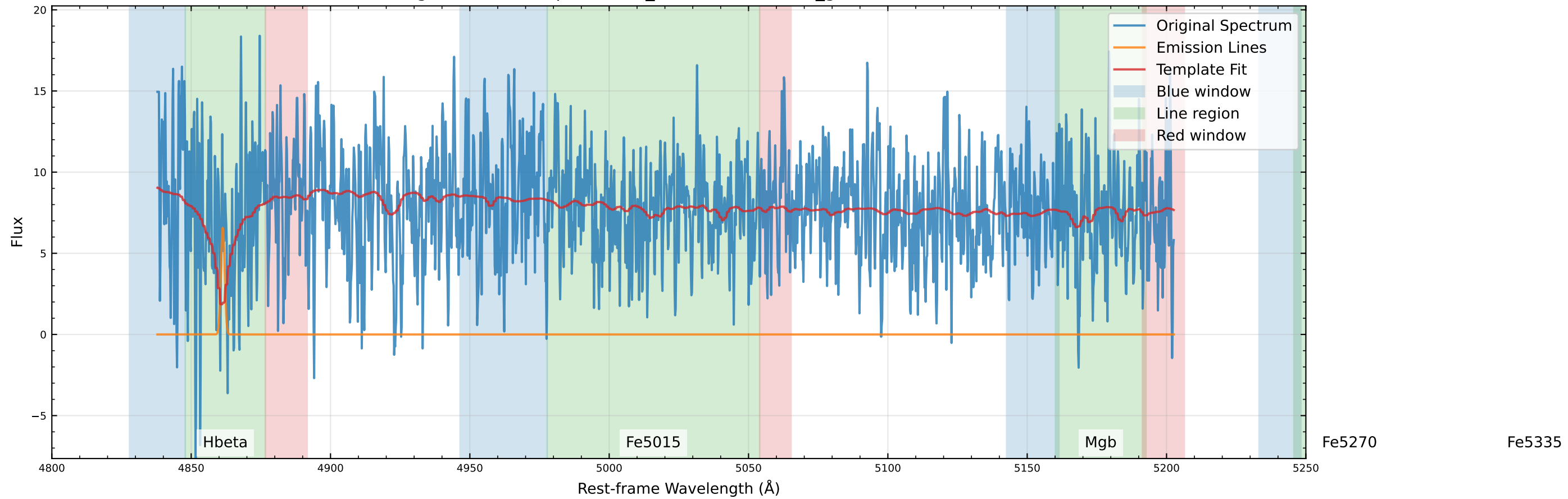
Original Data Comparison (v_star=43.5 km/s, v_gas=20.4 km/s)
