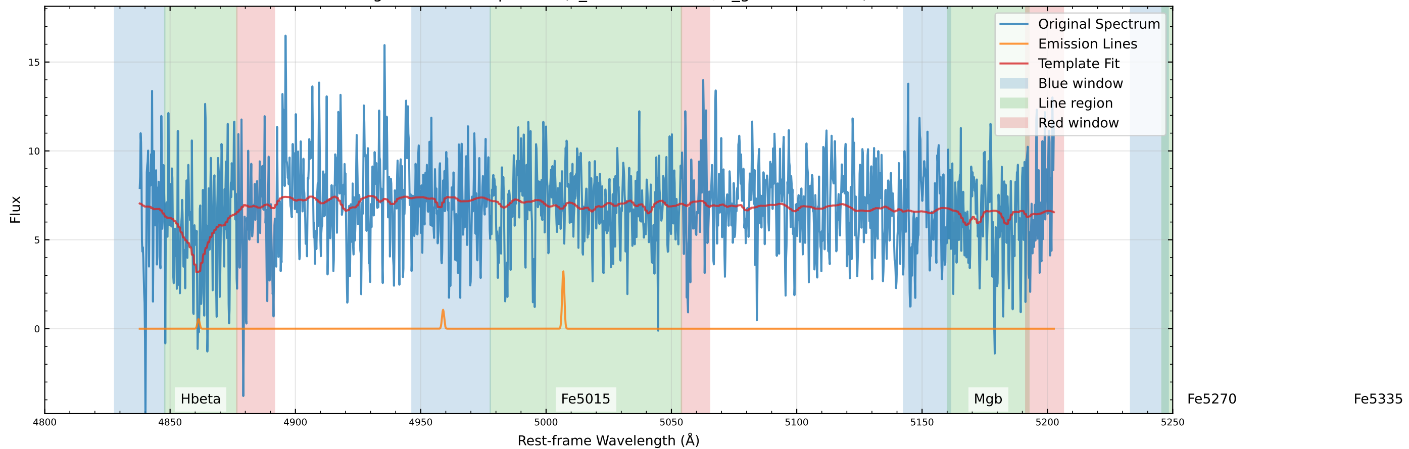
Original Data Comparison (v_star=44.6 km/s, v_gas=79.4 km/s)
