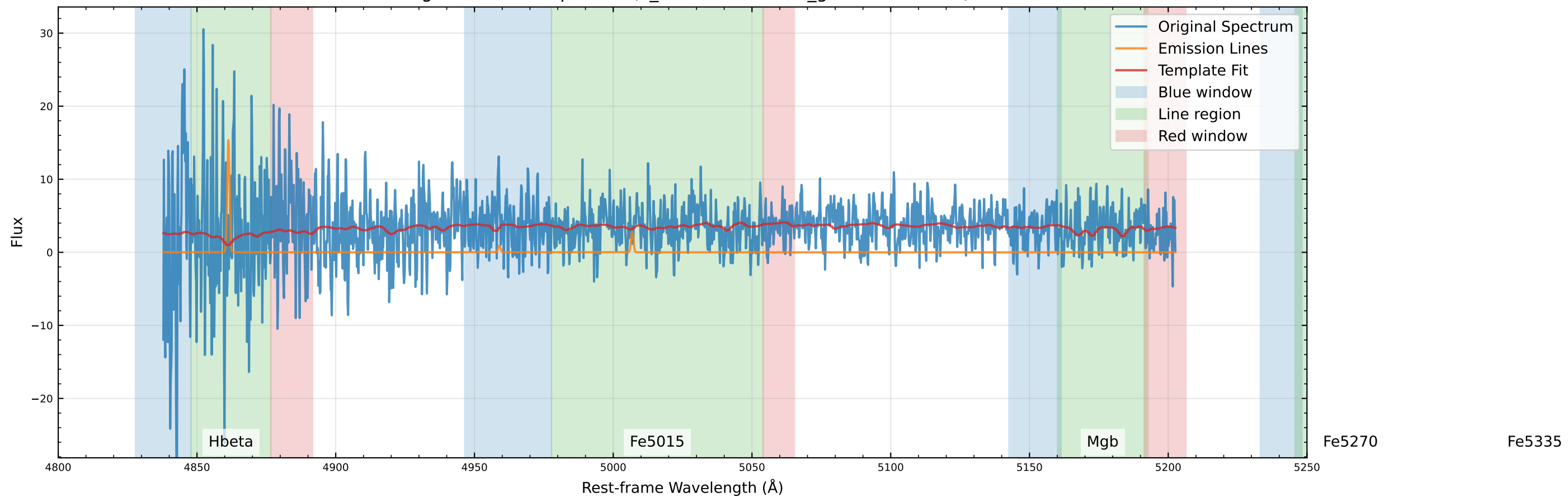
Original Data Comparison (v_star=2.2 km/s, v_gas=114.1 km/s)
