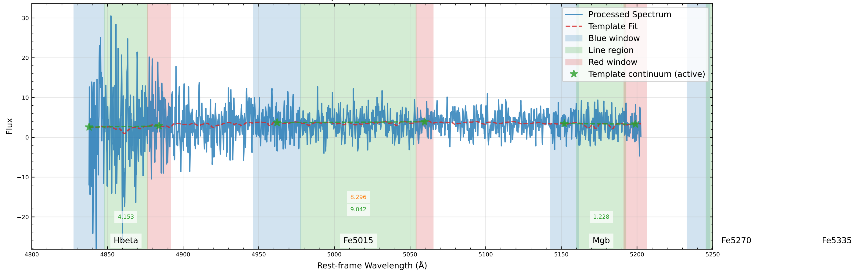
Processed Spectrum with Continuum Fits
