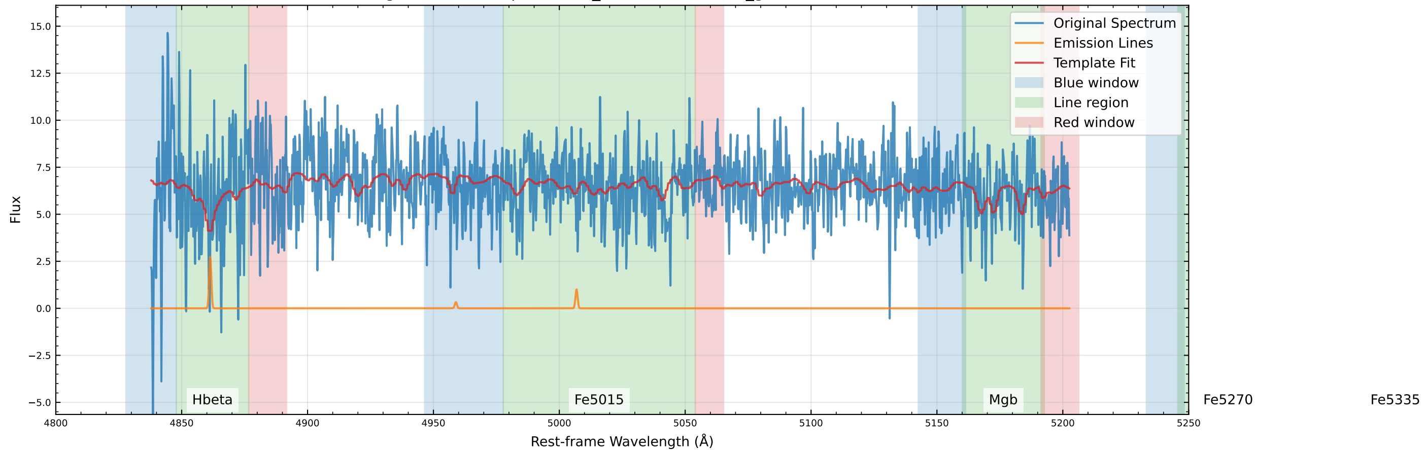
Original Data Comparison (v_star=27.8 km/s, v_gas=97.9 km/s)
