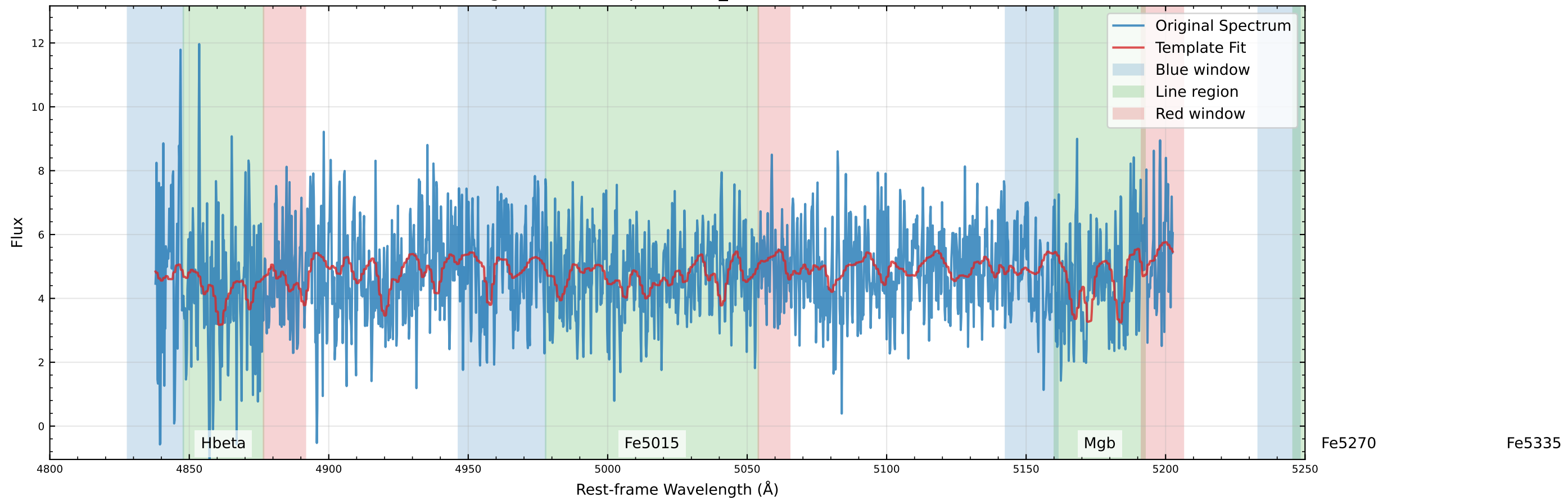
Original Data Comparison (v_star=-318.5 km/s)
