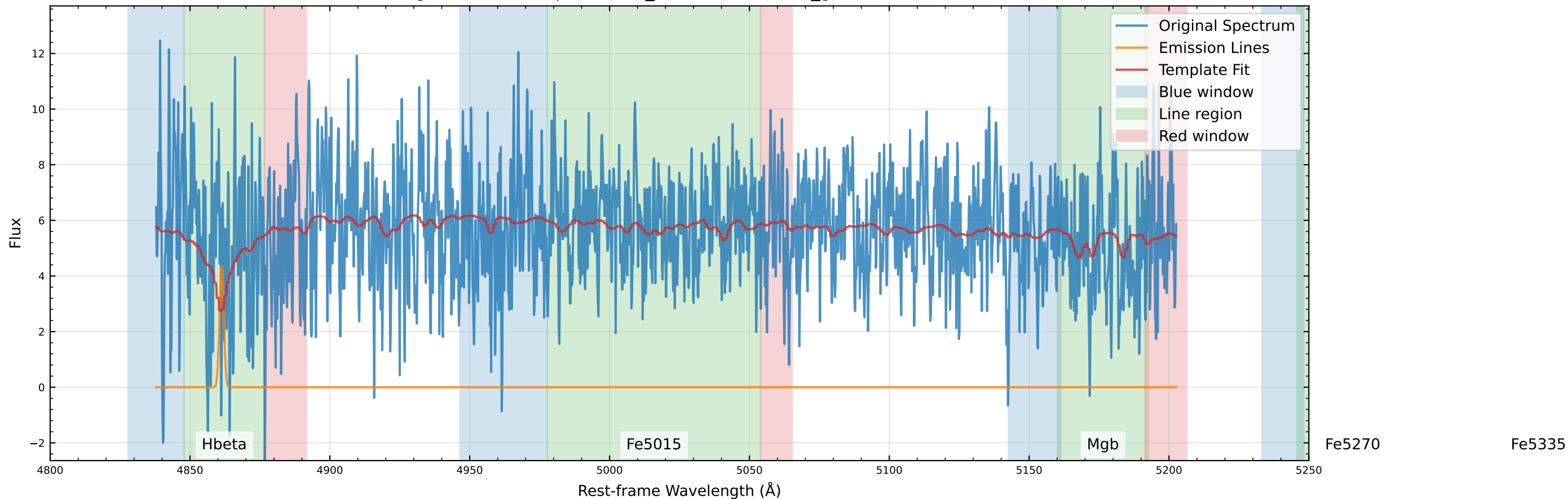
Original Data Comparison (v_star=-1.0 km/s, v_gas=-84.5 km/s)
