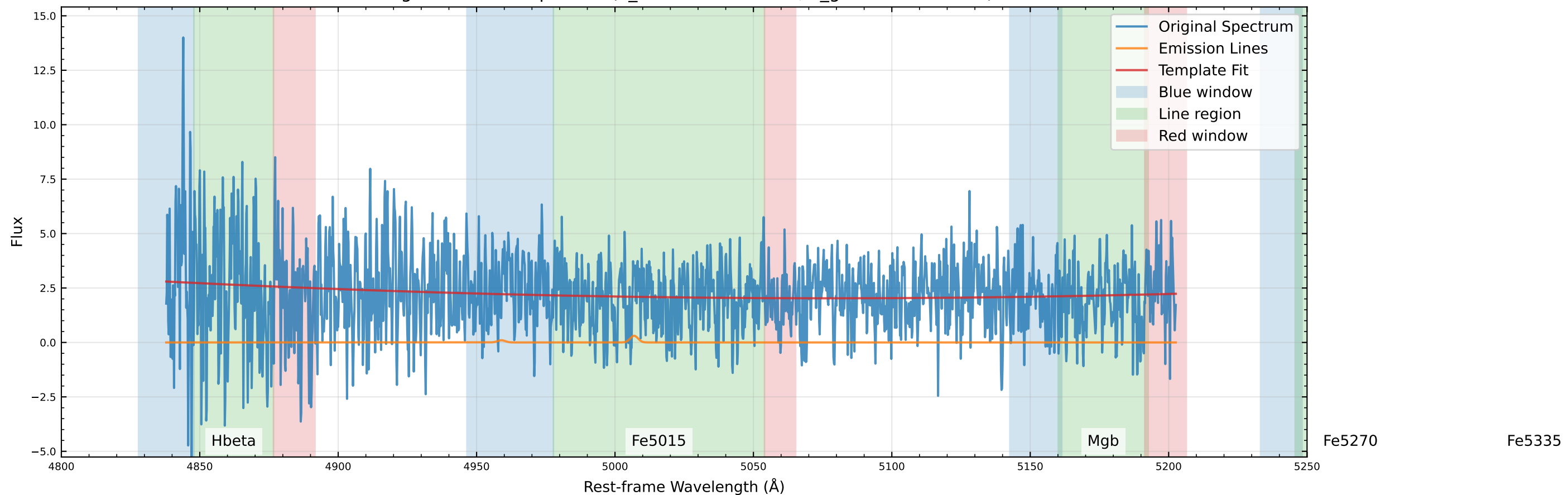
Original Data Comparison (v_star=1533.0 km/s, v_gas=1541.3 km/s)
