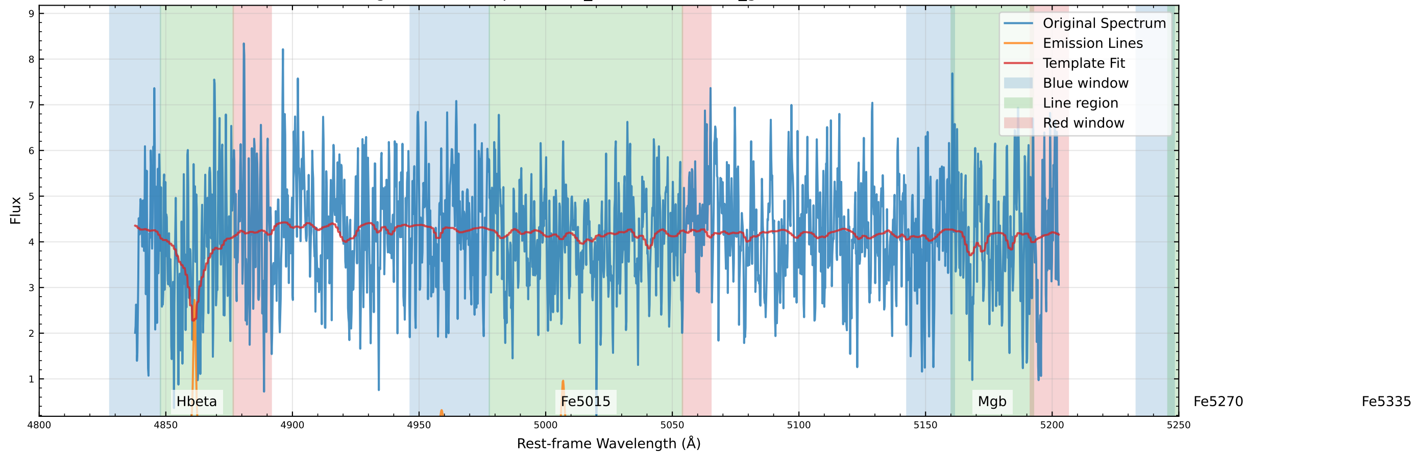
Original Data Comparison (v_star=24.2 km/s, v_gas=6.7 km/s)
