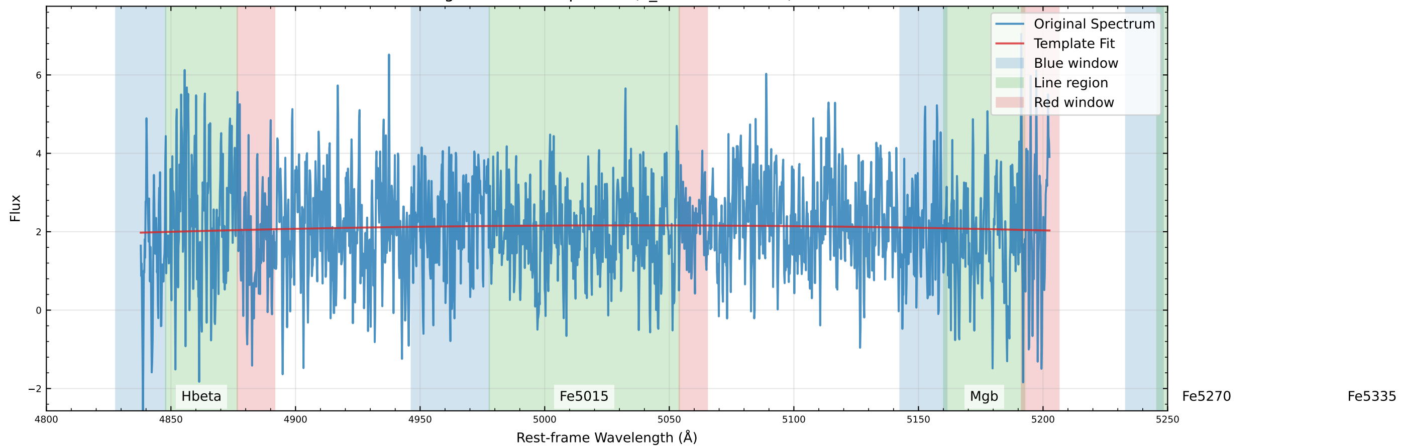
Original Data Comparison (v_star=-10.2 km/s)
