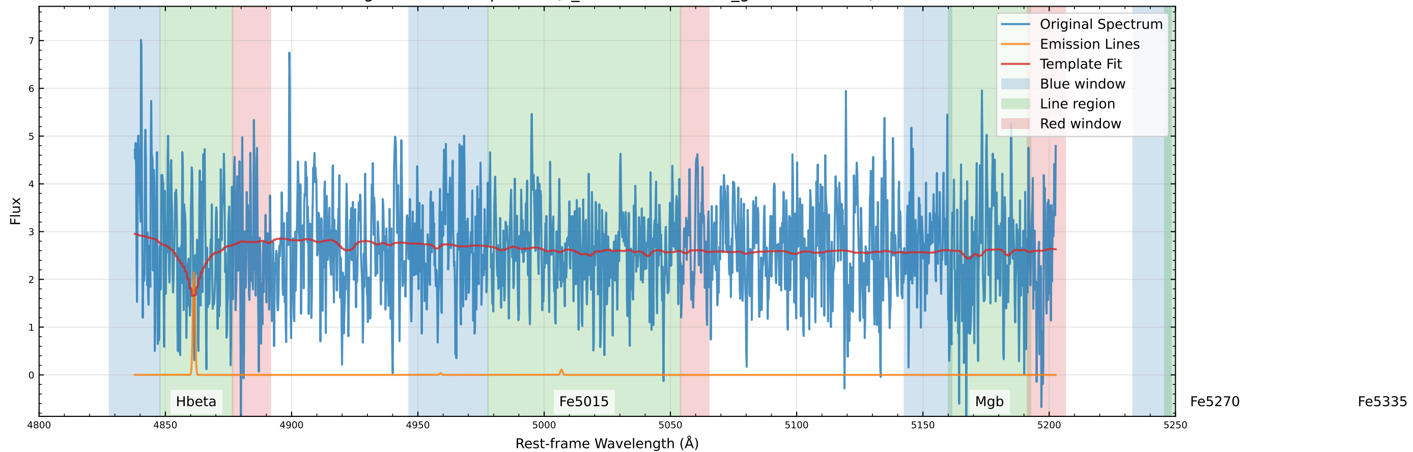
Original Data Comparison (v_star=-86.4 km/s, v_gas=-53.8 km/s)
