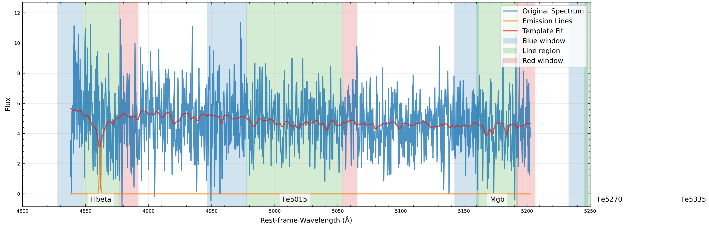
Original Data Comparison ( v_{\text{star}}=41.5 km/s, v_{\text{gas}}=106.2 km/s)
