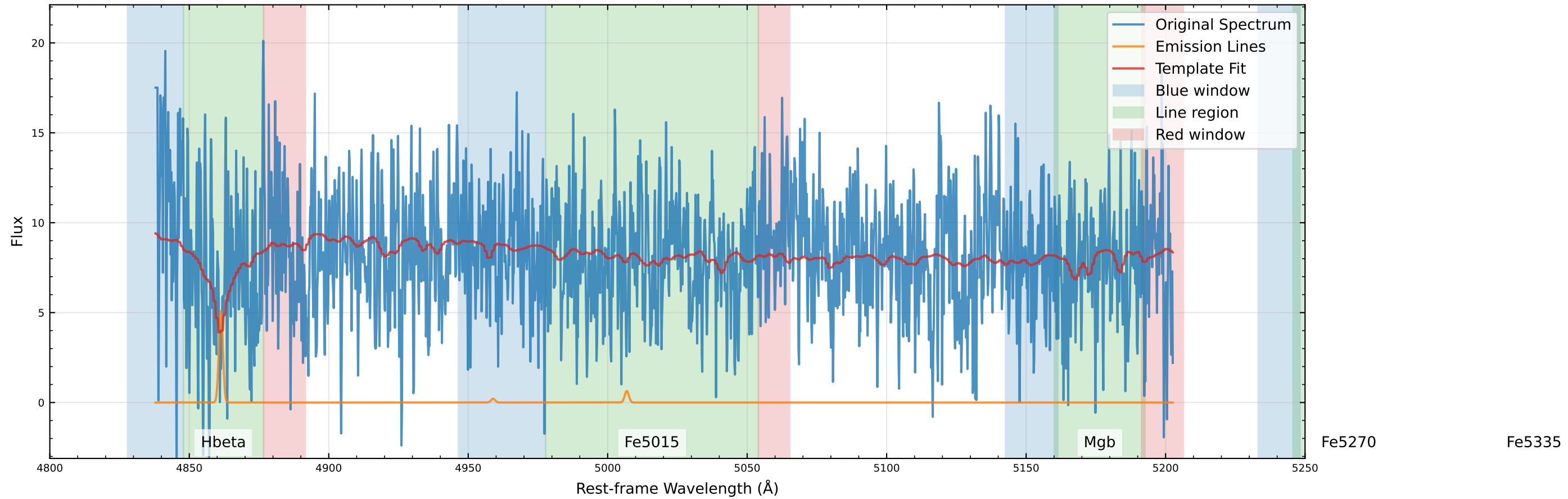
Original Data Comparison ( v_{\text{star}}=88.7 km/s, v_{\text{gas}}=112.2 km/s)
