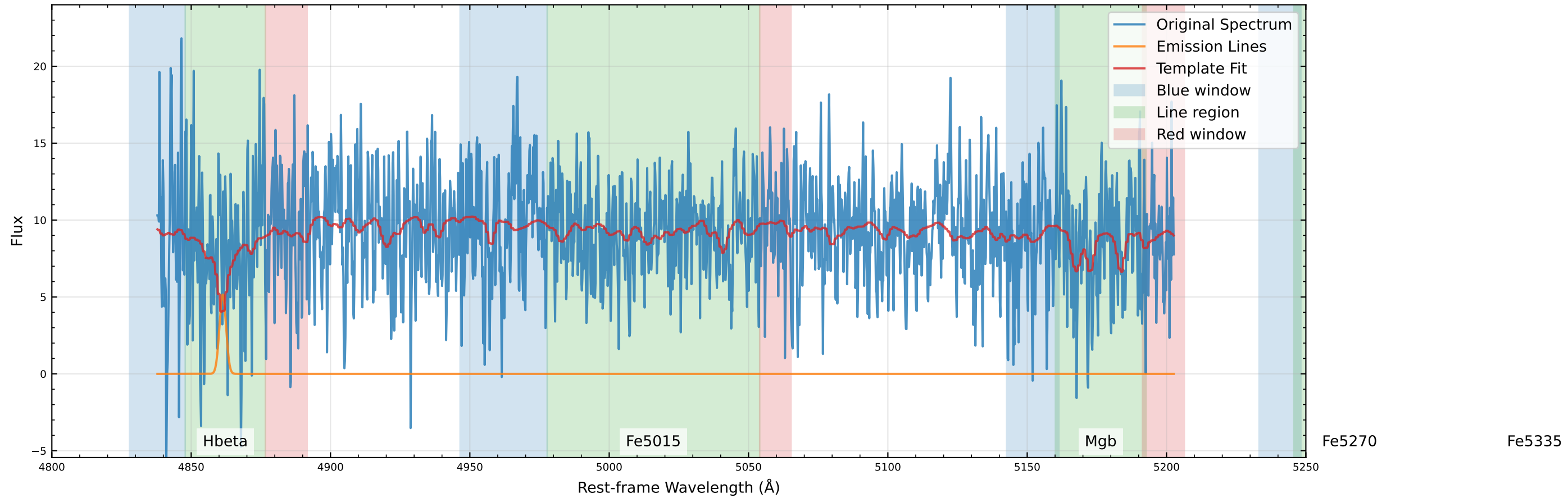
Original Data Comparison (v_star=49.6 km/s, v_gas=-7.6 km/s)
