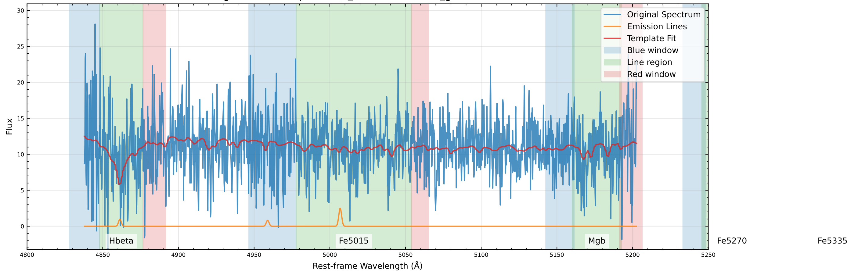
Original Data Comparison (v_star=56.4 km/s, v_gas=-14.5 km/s)
