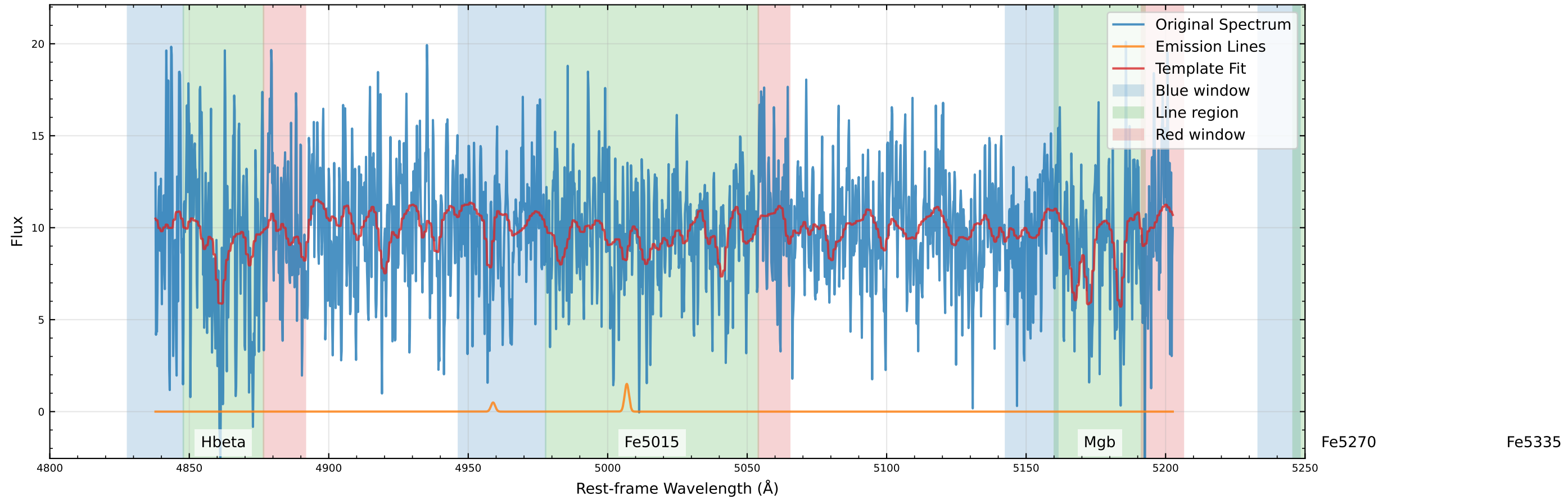
Original Data Comparison (v_star=6.6 km/s, v_gas=35.0 km/s)
