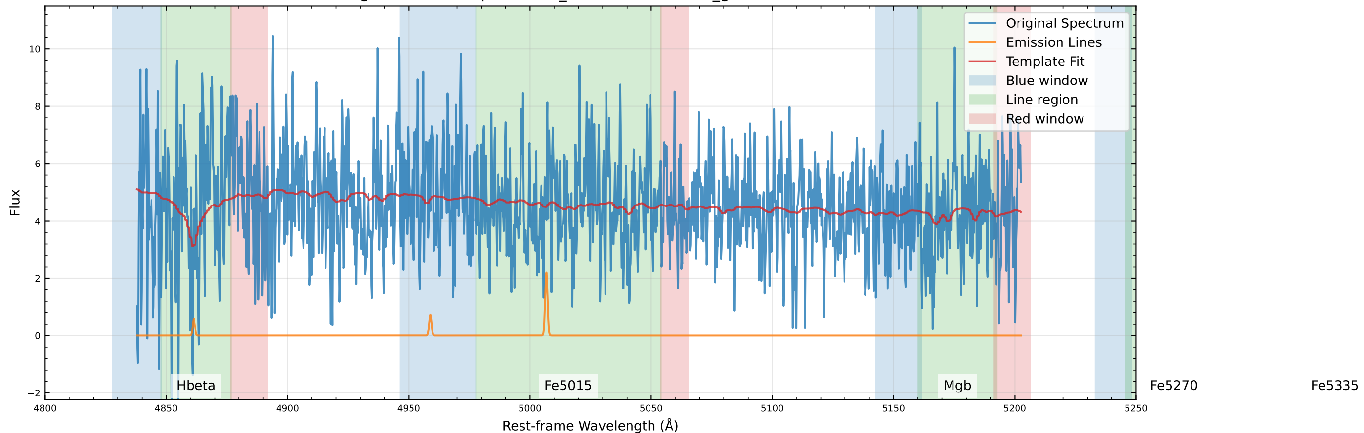
Original Data Comparison (v_star=-43.5 km/s, v_gas=41.8 km/s)
