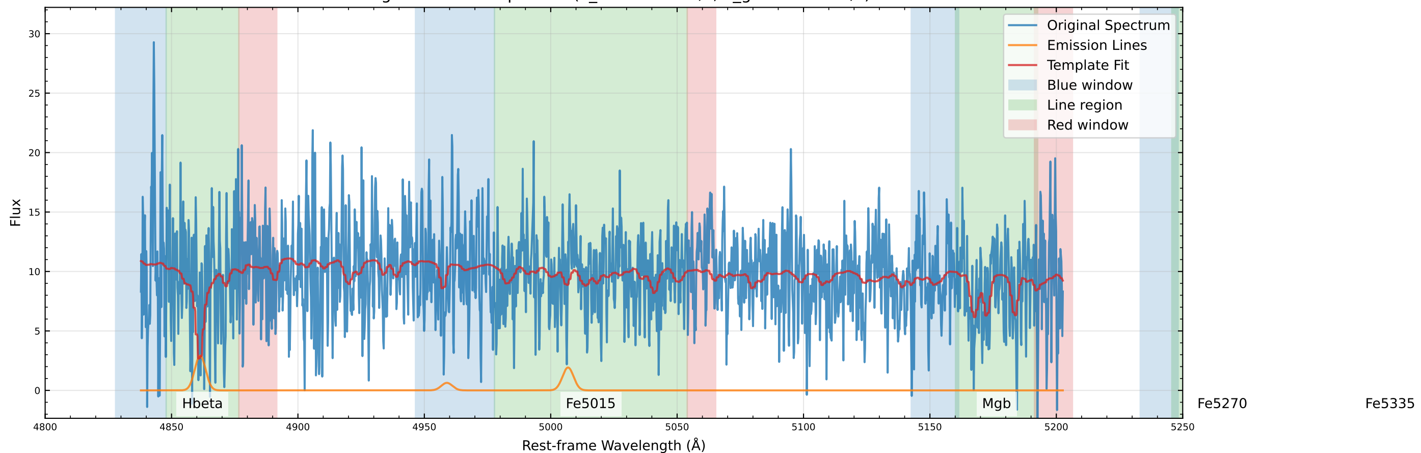
Original Data Comparison (v_star=1.0 km/s, v_gas=56.9 km/s)
