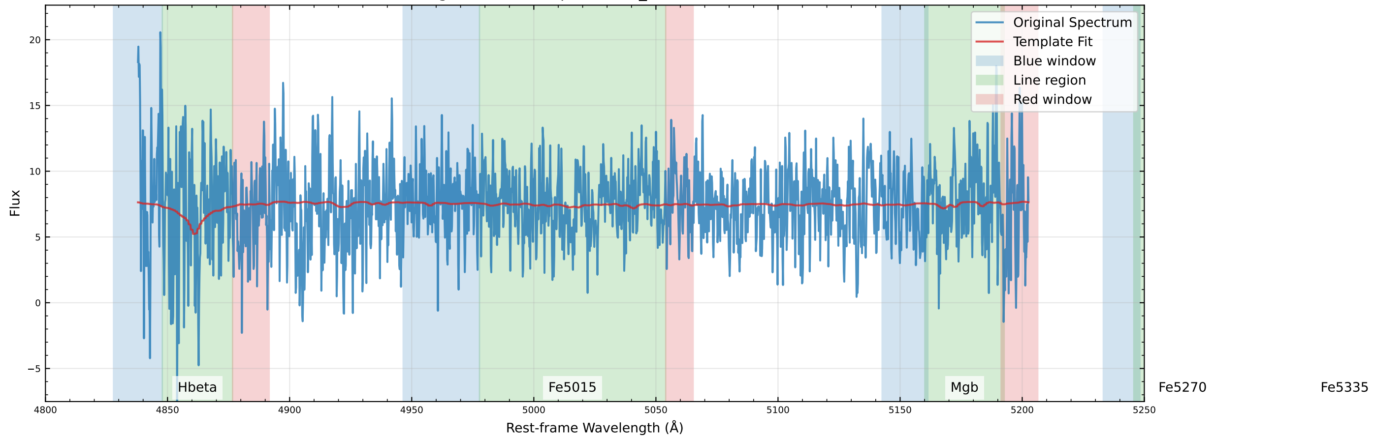
Original Data Comparison (v_star=55.4 km/s)
