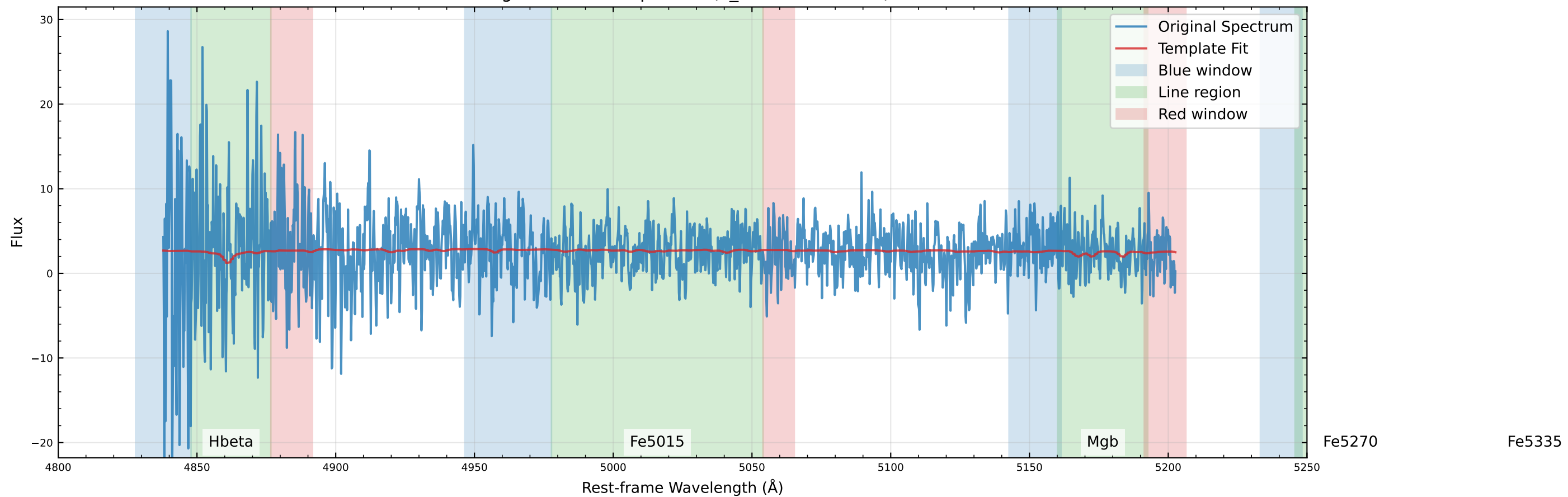
Original Data Comparison (v_star=-37.7 km/s)
