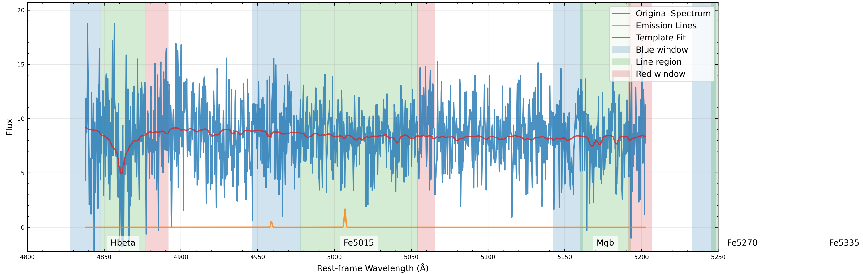
Original Data Comparison (v_star=63.2 km/s, v_gas=75.5 km/s)
