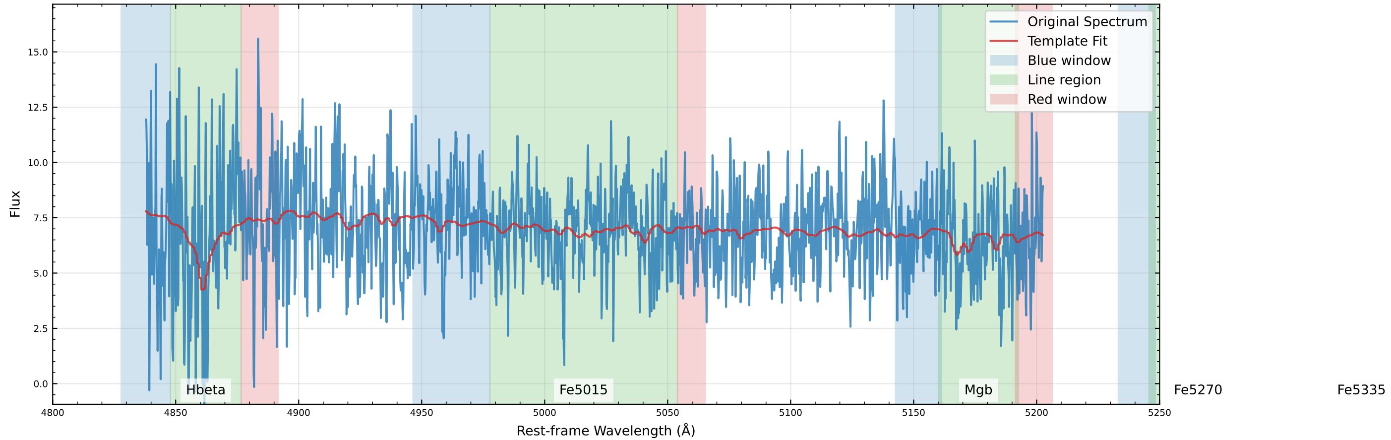
Original Data Comparison (v_star=75.6 km/s)
